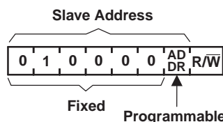
Figure 4. TCA6408 Address
